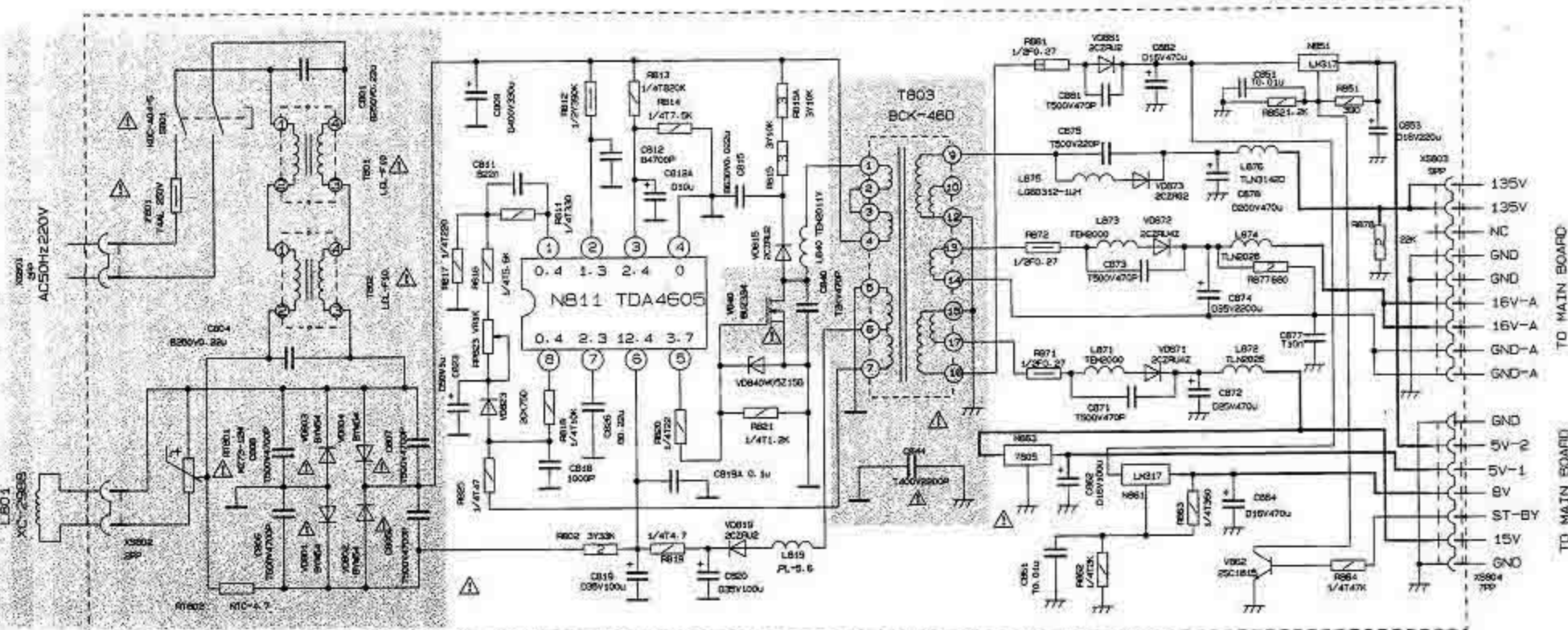
POWER BOARD JUC7.820.028
