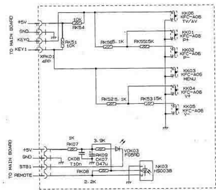
K BOARD JUC7.820.116
