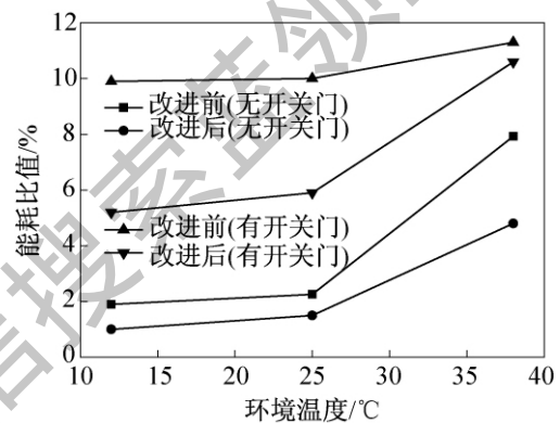
图8 改进前后化霜能耗占总能耗的比值 Fig.8 The percentage of defrosting energy consumption in total energy consumption
