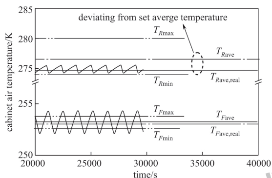
(a) temperature fluctuation under sequential control strategy
