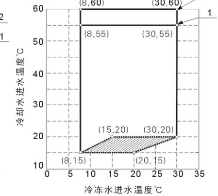
WPS.CFFHT启动范围
