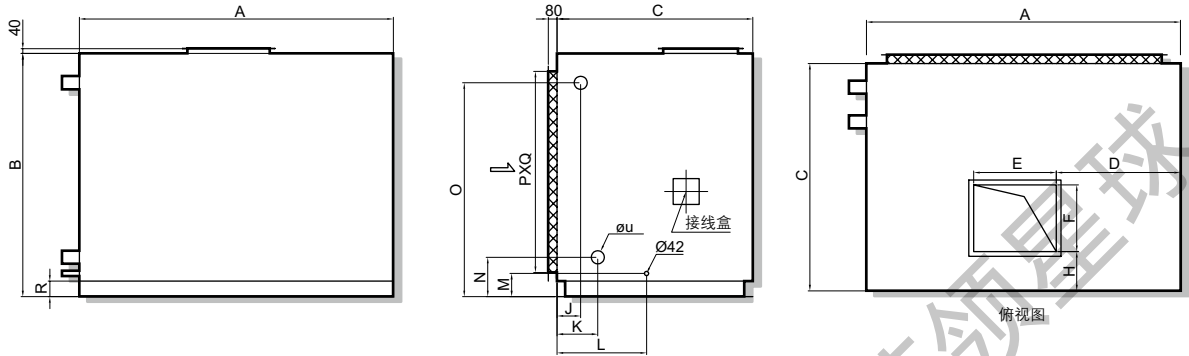
卧式顶出风
