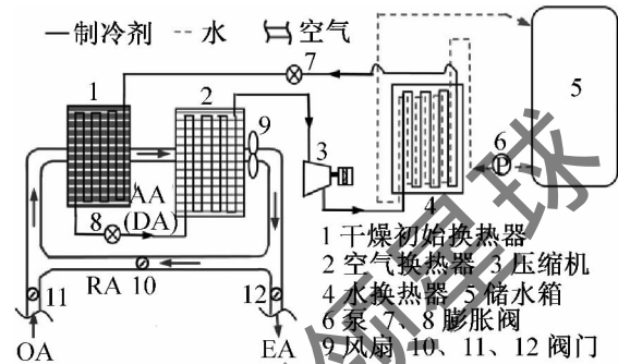
图5 无霜空气源热泵热水器原理图 Fig. 5 Schematic diagram of the frost-free air source heat pump system
