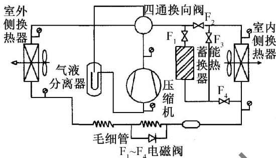
图4 空气源热泵蓄能热气除霜系统 Fig. 4 Schematic of PCM based thermal energy storage and defrosting for air source heat pump
