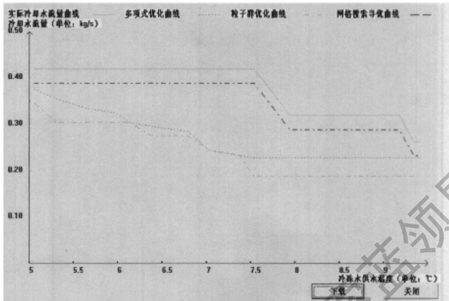
图 5.20 60%冷负荷, 环境湿球温度为 25℃下冷却水质量流量设定点的优化 Fig.5.20 60 percent of cooling load, environment humid ball temperature 25℃, the setpoint optimization of cooling water flow
